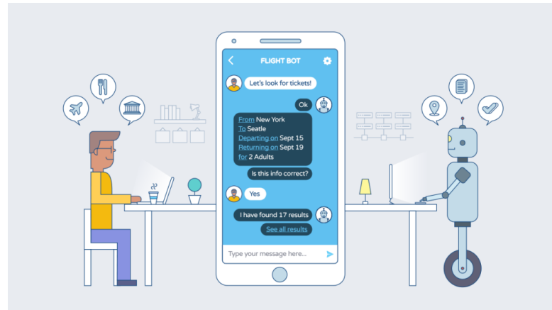
Text-based chatbot
